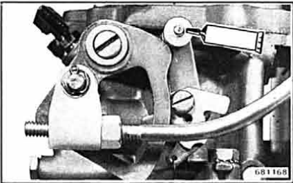
Figure 2-5. Carburetor Linkage
