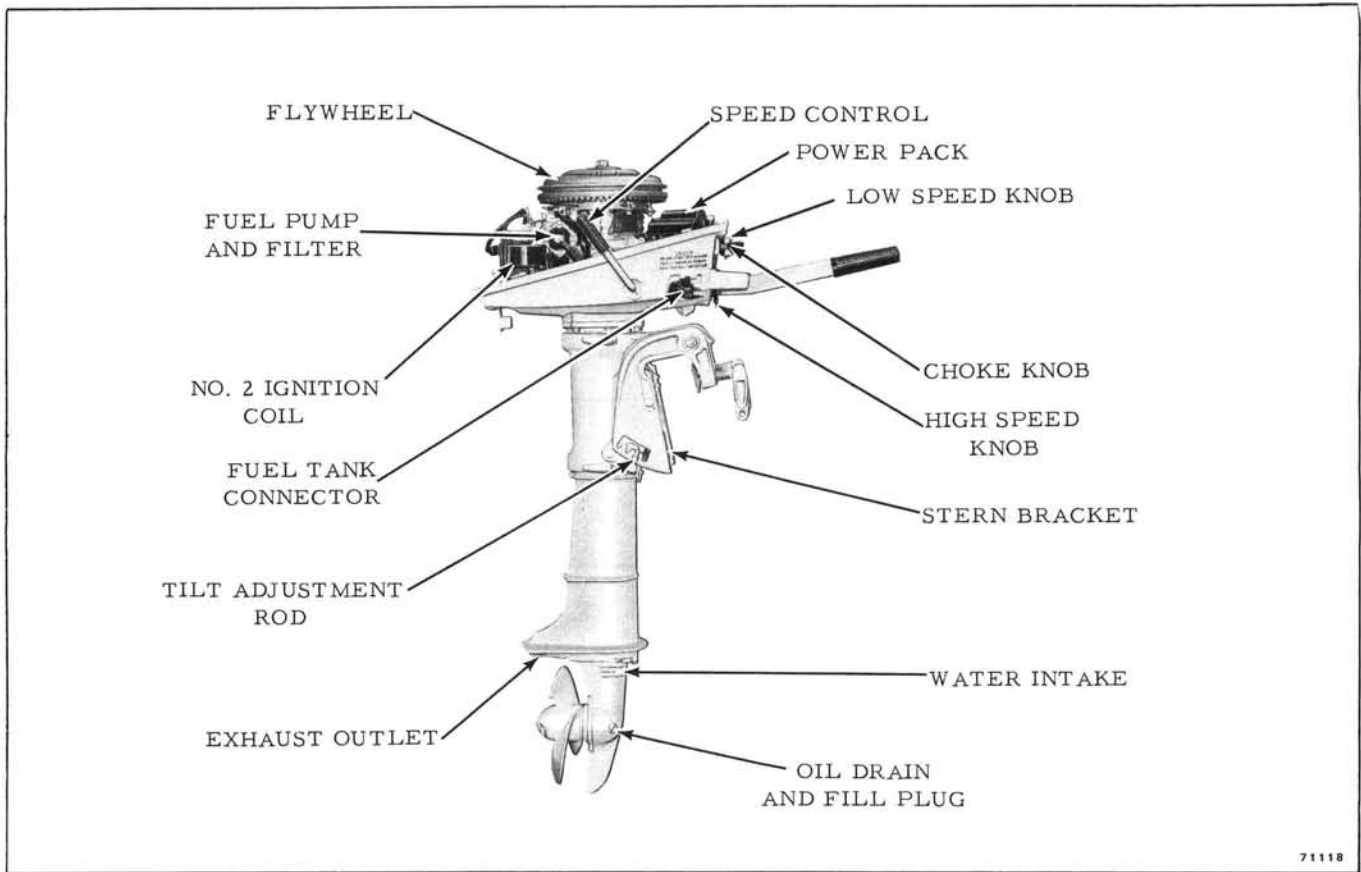
Figure 1-1. 4 H.P. with Standard Gearcase - Starboard Side
